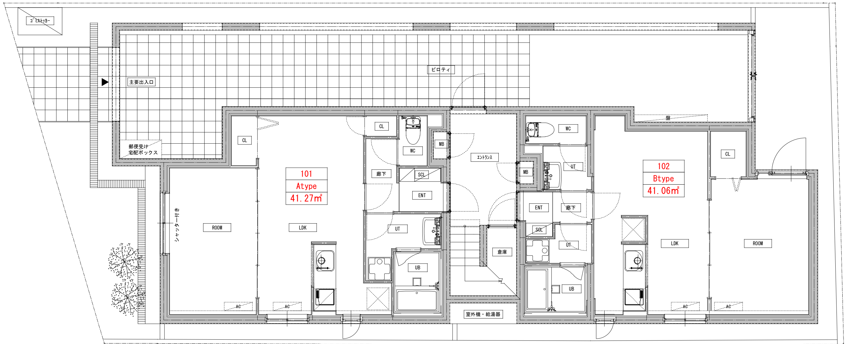
1階平面図S=1/60
